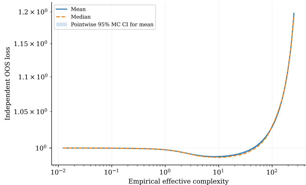
heteroskedastic, T=1440
